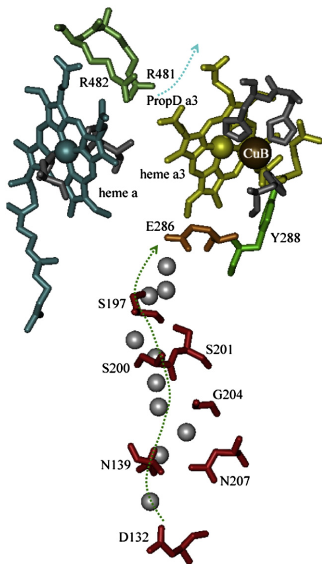
Fig. 1. Active site and D-channel of cytochrome c oxidase from R. sphaeroides (PDB ID 1M56, Ref. [36]). Key active-site residues and cofactors include heme a3 (yellow), \text{Cu}_\text{B} (tan) with its three ligated histidines (gray), Y288 (green), E286 (orange), R481 and R482 (lime), heme a (cyan), H421, and H102 (gray). A light-blue arrow indicates a putative proton exit pathway starting at the R481-PropD salt-link. A green arrow connects D132 at the entrance to E286 at the top of the D-channel, with intervening residues in red and crystallographic water in white.
